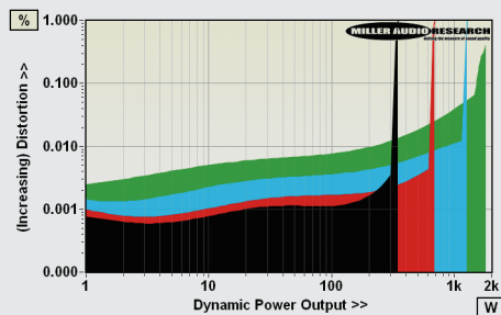
ABOVE: Dynamic power output versus distortion into 8ohm (black trace), 4ohm (red), 2ohm (blue) and 1ohm (green) speaker loads. Max. current is 42.7A
